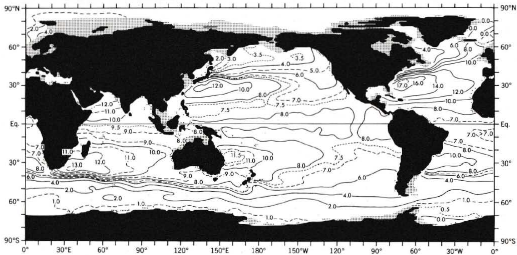
FIGURE 8.5. Global distribution of the annual-mean temperature in °C at 500-m depth (from Levitus, 1982).
