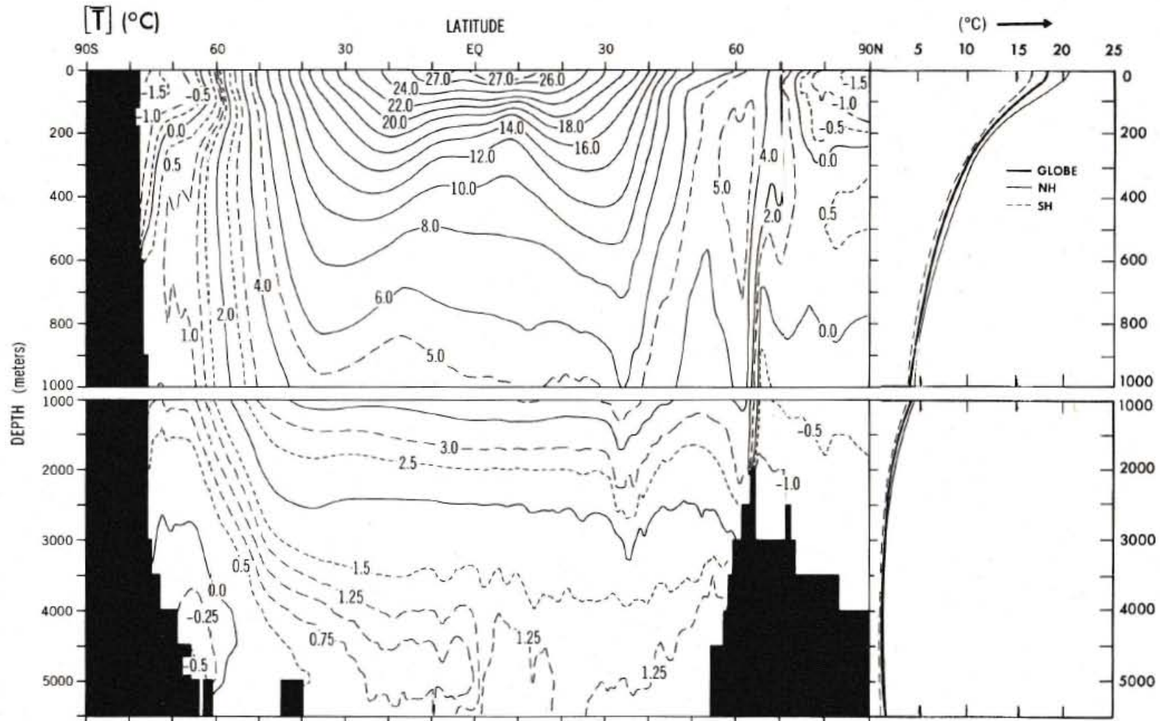
FIGURE 8.4. Zonal-mean cross section of temperature for the top ocean layer 0–1000 m and the layer below 1000 m in °C for annual-mean conditions. Vertical profiles of the hemispheric and global mean temperatures are shown on the right (after Levitus, 1982).
